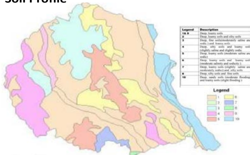
Soil Profile
